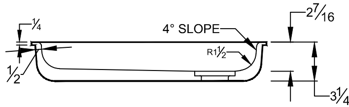
SECTION VIEW
