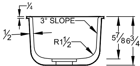
SECTION VIEW
