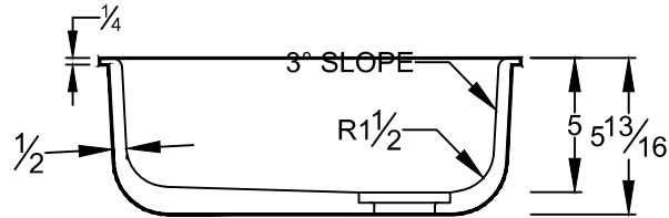
SECTION VIEW
