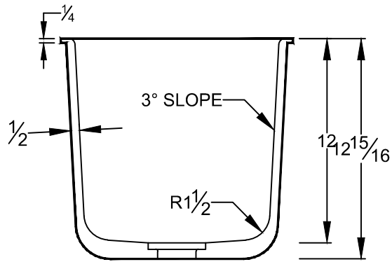
SECTION VIEW
