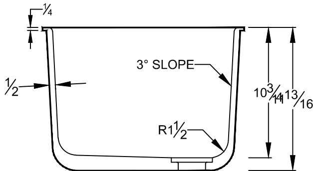
SECTION VIEW
