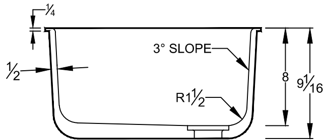
SECTION VIEW
