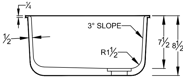
SECTION VIEW
