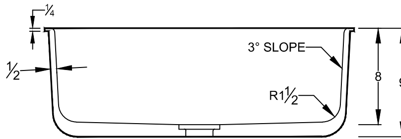
SECTION VIEW
