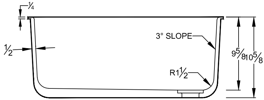
SECTION VIEW
