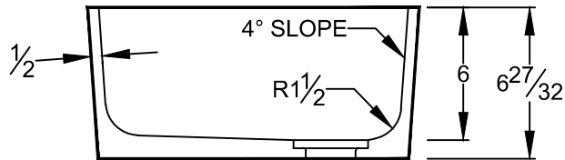
SECTION VIEW
