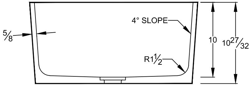
SECTION VIEW
