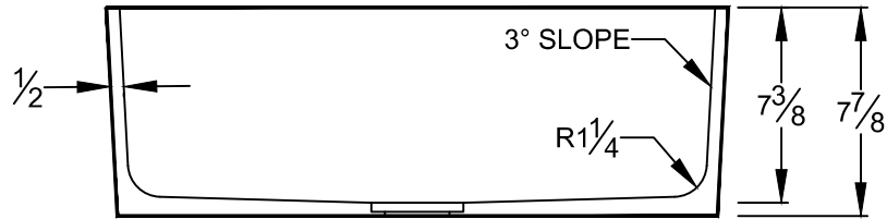
SECTION VIEW
