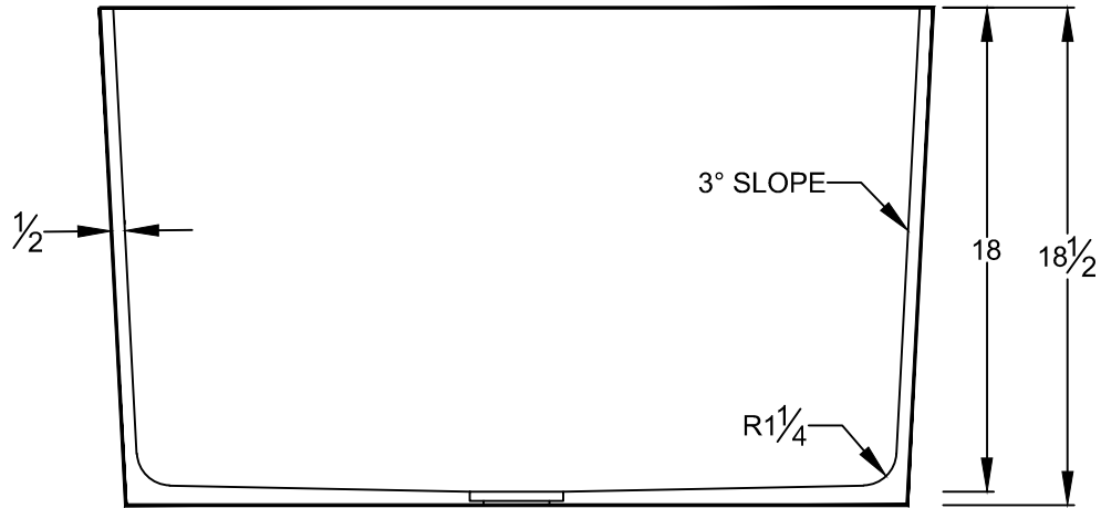
SECTION VIEW
