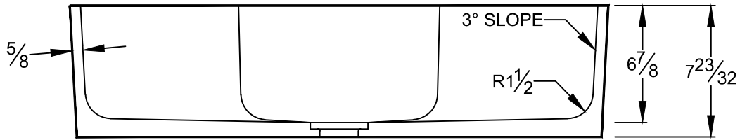
SECTION VIEW
