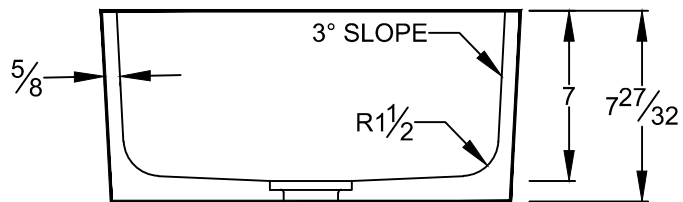
SECTION VIEW
