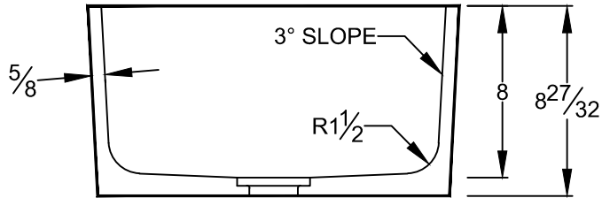
SECTION VIEW
