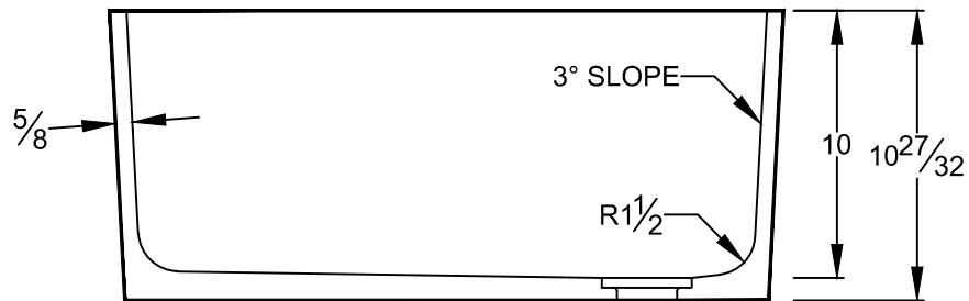
SECTION VIEW
