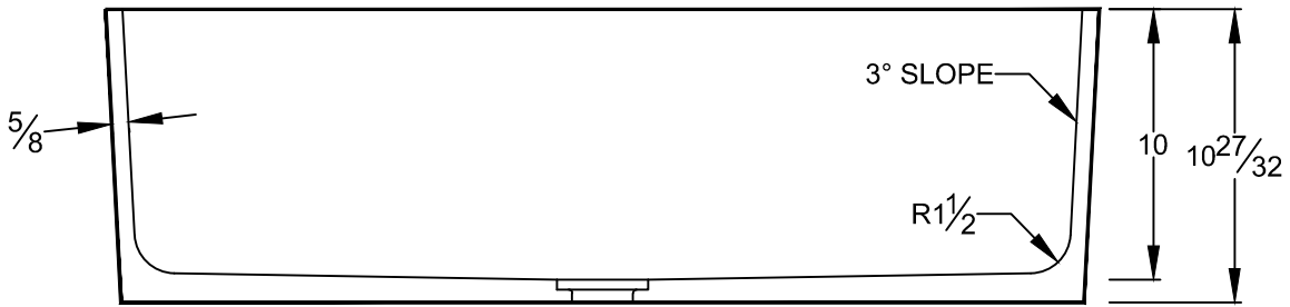
SECTION VIEW
