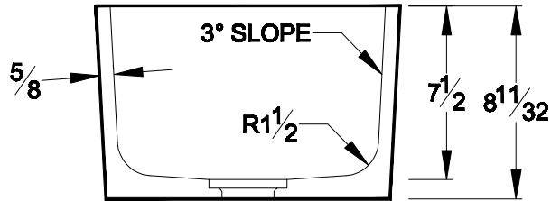
SECTION VIEW
