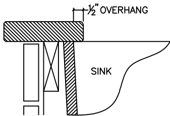
INSTALLATION DETAIL
