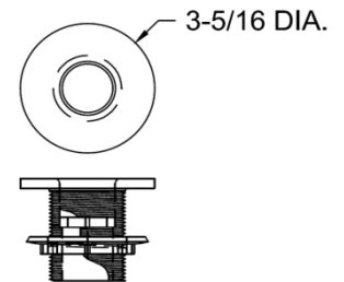
PSO3R SINK OUTLET WITH INTEGRAL TAILPIECE 1 1/2" N.P.T.
