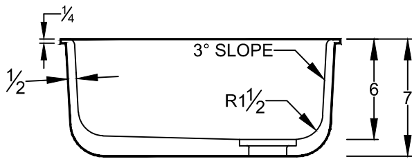
SECTION VIEW
