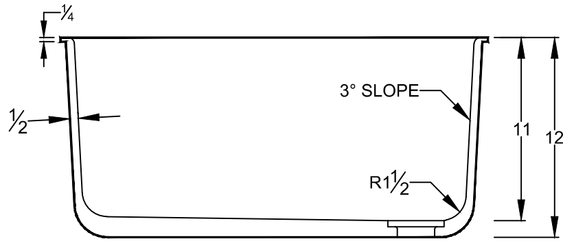
SECTION VIEW
