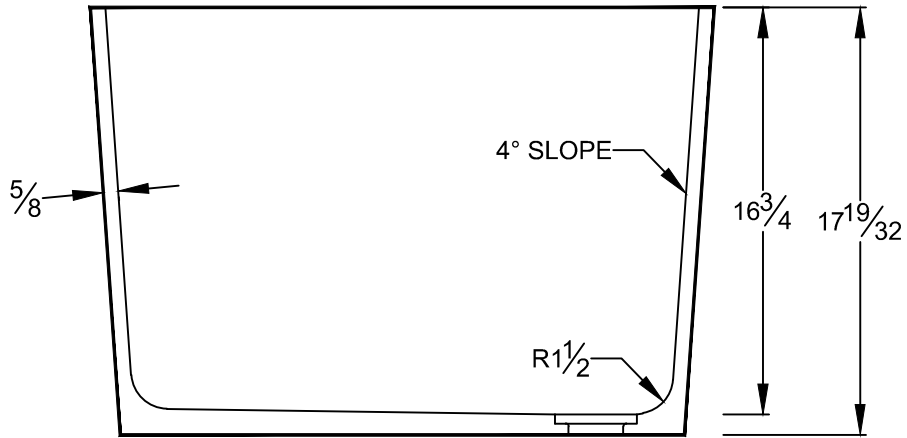
SECTION VIEW
