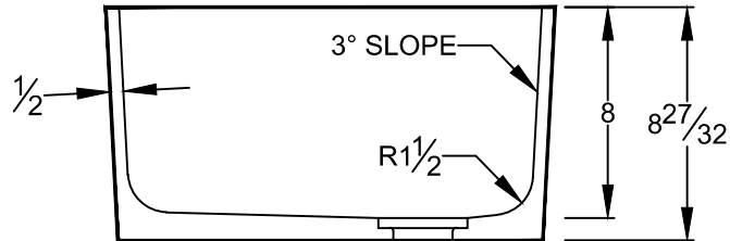
SECTION VIEW
