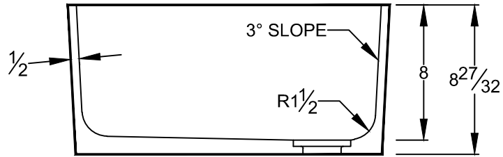
SECTION VIEW
