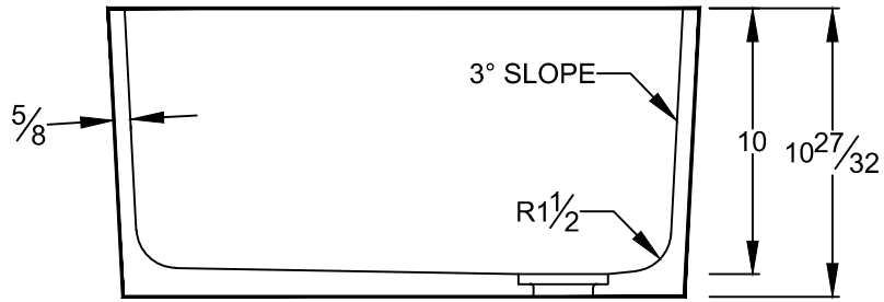
SECTION VIEW
