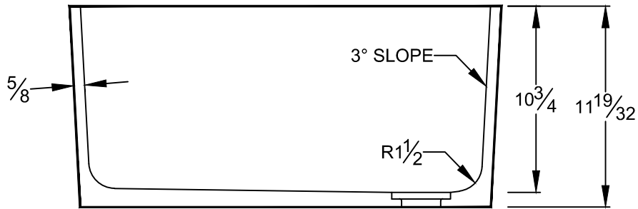
SECTION VIEW
