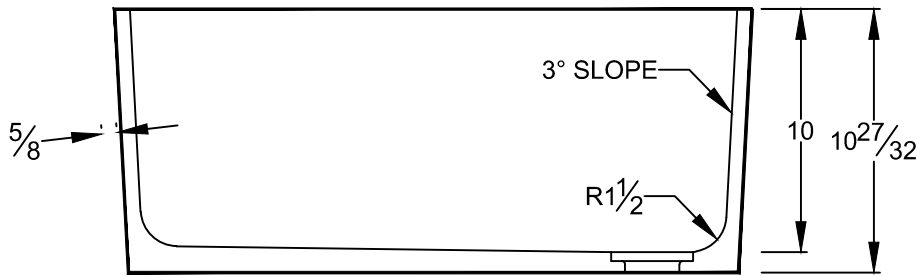
SECTION VIEW
