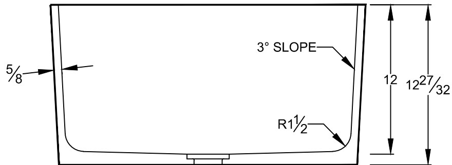
SECTION VIEW
