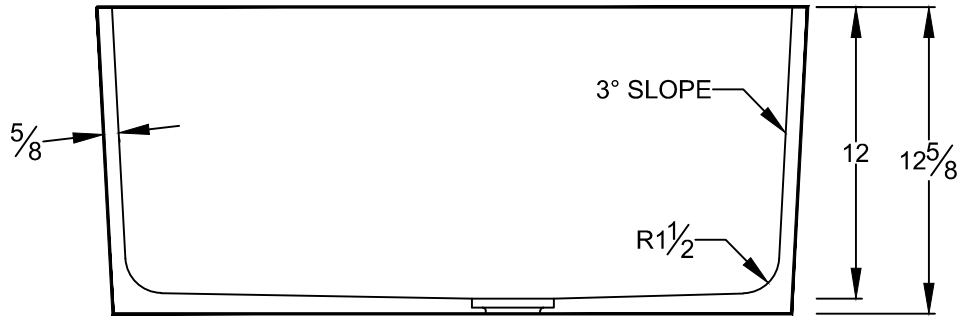
SECTION VIEW
