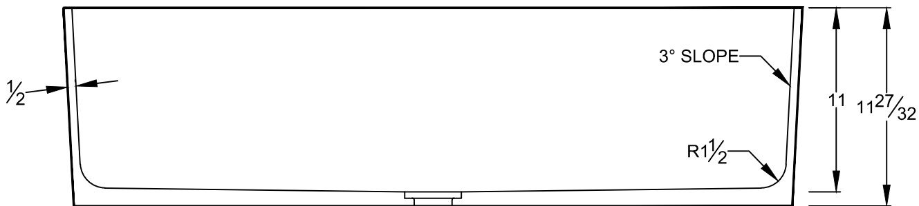
SECTION VIEW
