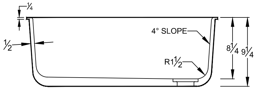
SECTION VIEW
